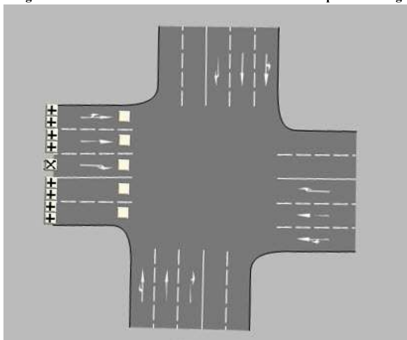
Figure 3: Intersection turns within VISUM for mesoscopic modelling
