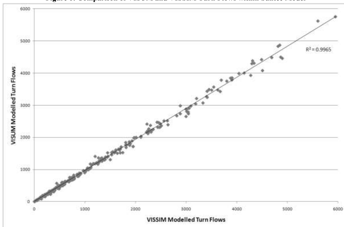
Figure 6: Comparison of VISUM and VISSIM Turn Flows within Suntec Model
