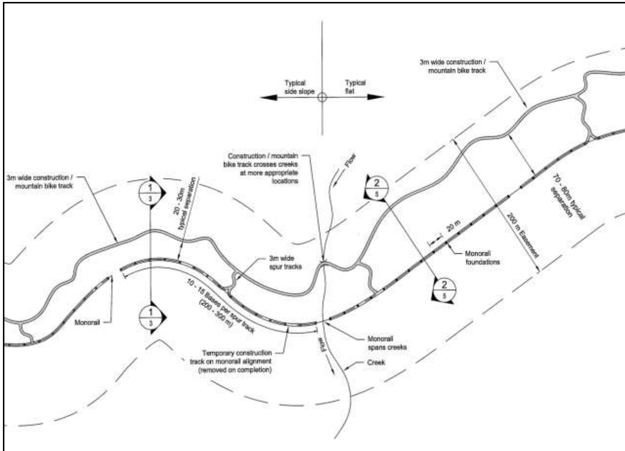
Figure 8: Indicative layout of monorail and mountain bike track
