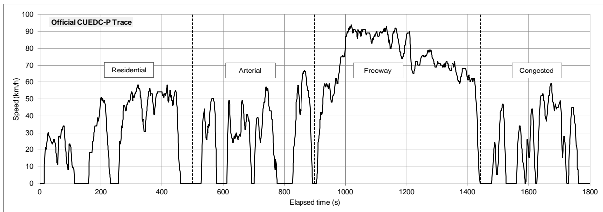
Figure 3 – CUEDC-P Driving Cycle
