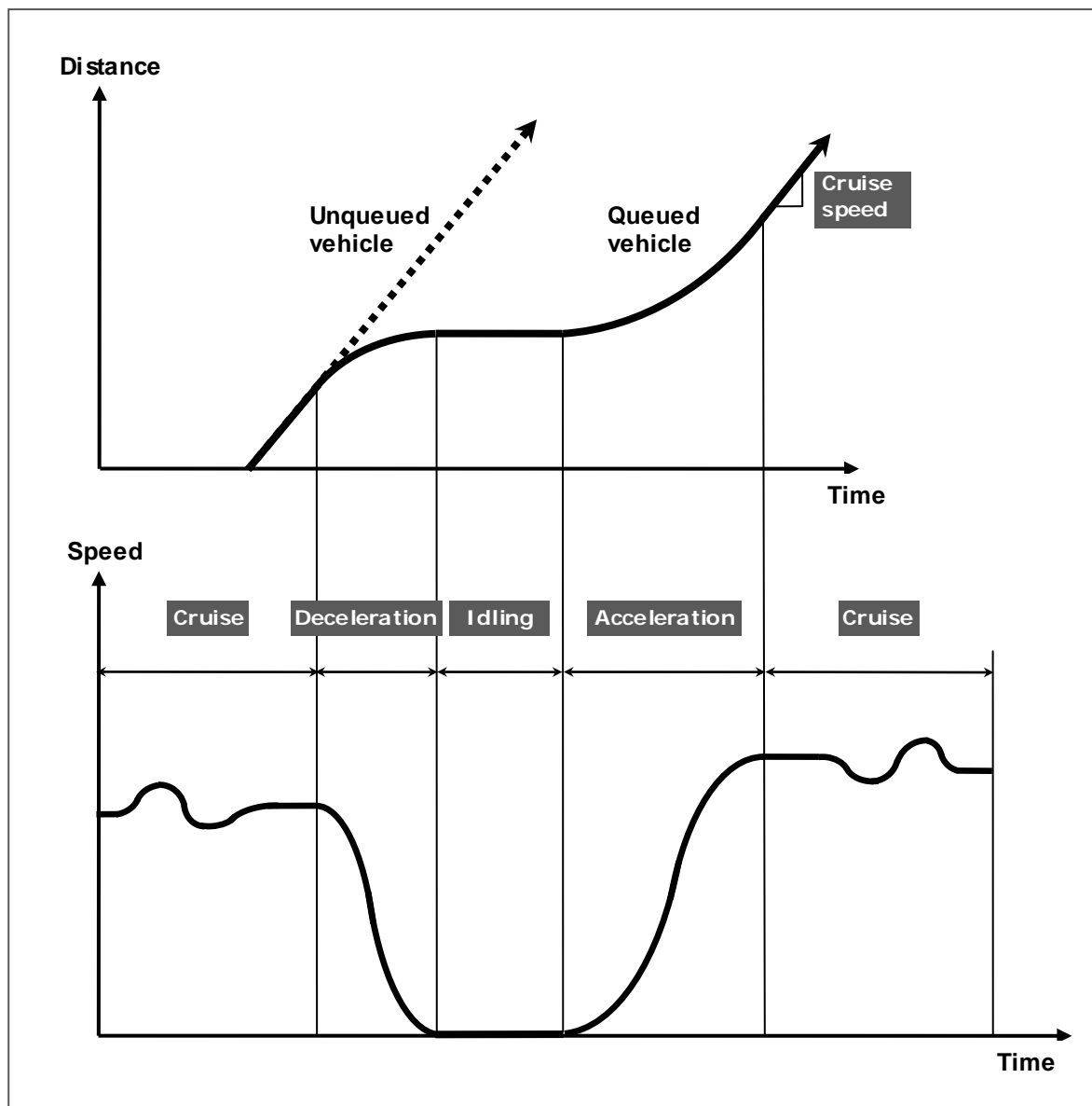
Figure 1 - Drive cycle during a stop - start manoeuvre (example)
