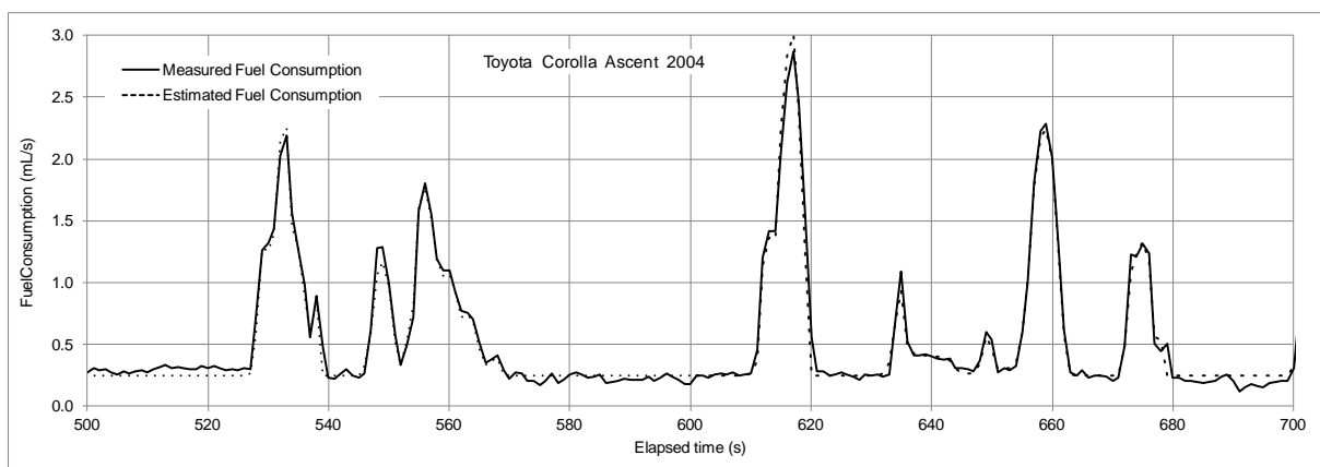
Figure 5 – Sample of time profiles of estimated and measured values of instantaneous fuel consumption rates
