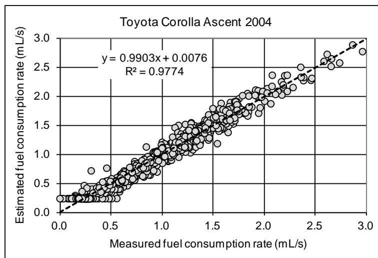
Figure 4 – Estimated vs measured values of instantaneous fuel consumption rates
